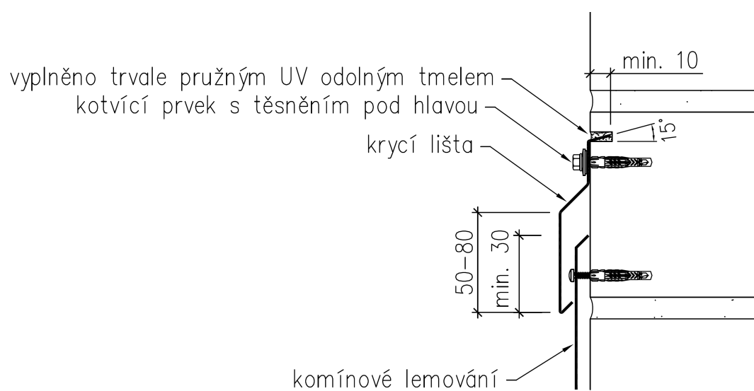
Obr. 17e: Detail C
